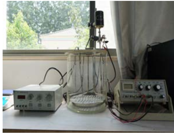
Insulator Tester
